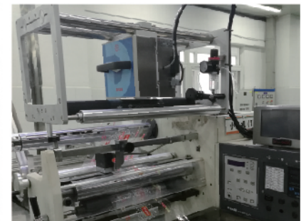
D03S installed on FFS Machine
