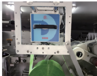
D03S installed on FFS Machine
